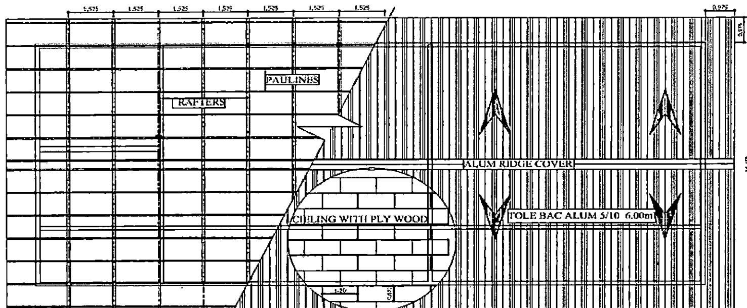
ROOF PLAN
